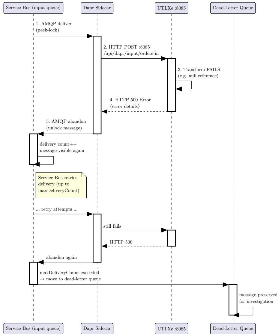
Figure 3: Rainy day: transformation fails → retry → dead-letter queue
